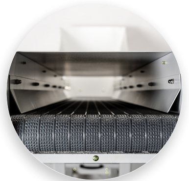
16" wide rubber conveyor belt removes shredded waste.
